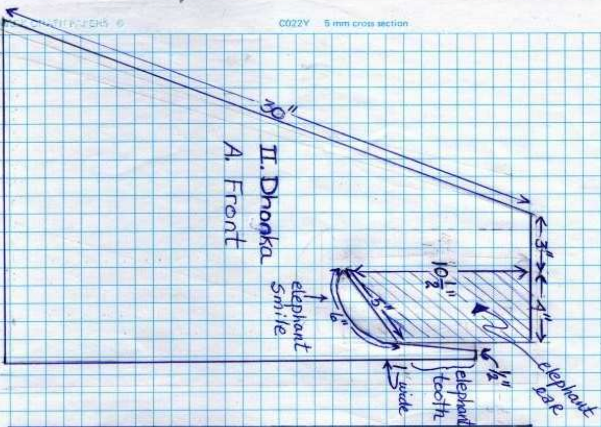
II Dhonka Diagram II.2 Drawn to scale 0.5cm = 2 inches
